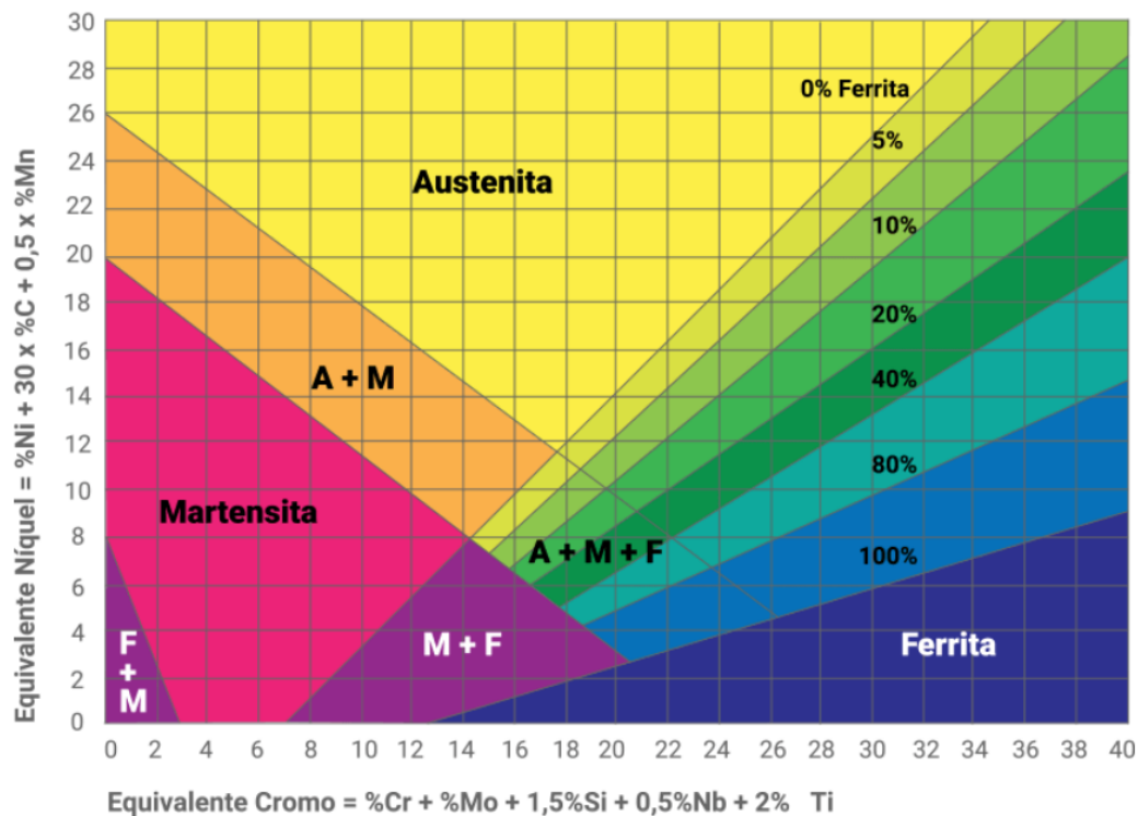
Figura 4. Diagrama de Schaeffler [10]
